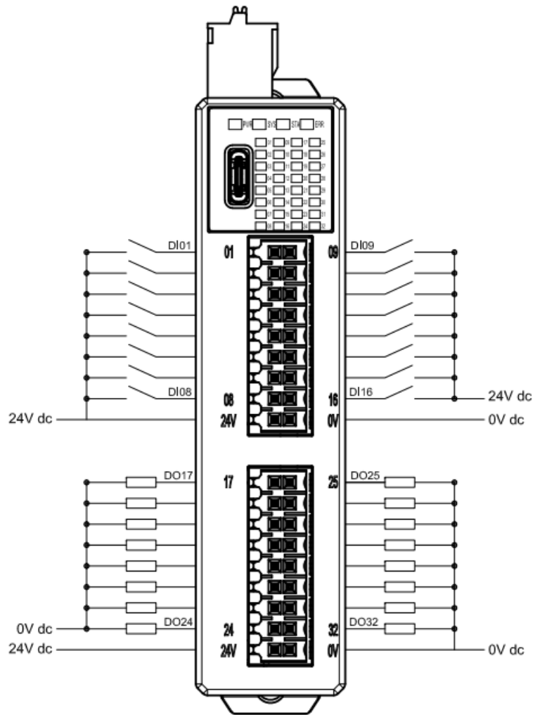
Fig 5. 7 GFNC-2A4A Wiring Diagram
