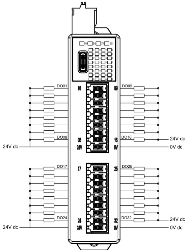
Fig 5. 4 GFNC-3A3A Wiring Diagram
