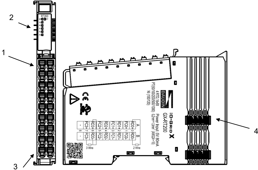
Figure 3.1 GX-RT200
