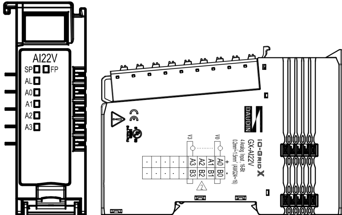
Figure 4.19 GX-AI22V Wiring Diagram
