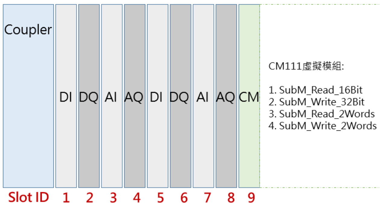
Figure 9.11 Configuration Diagram of Simulated System Modules
