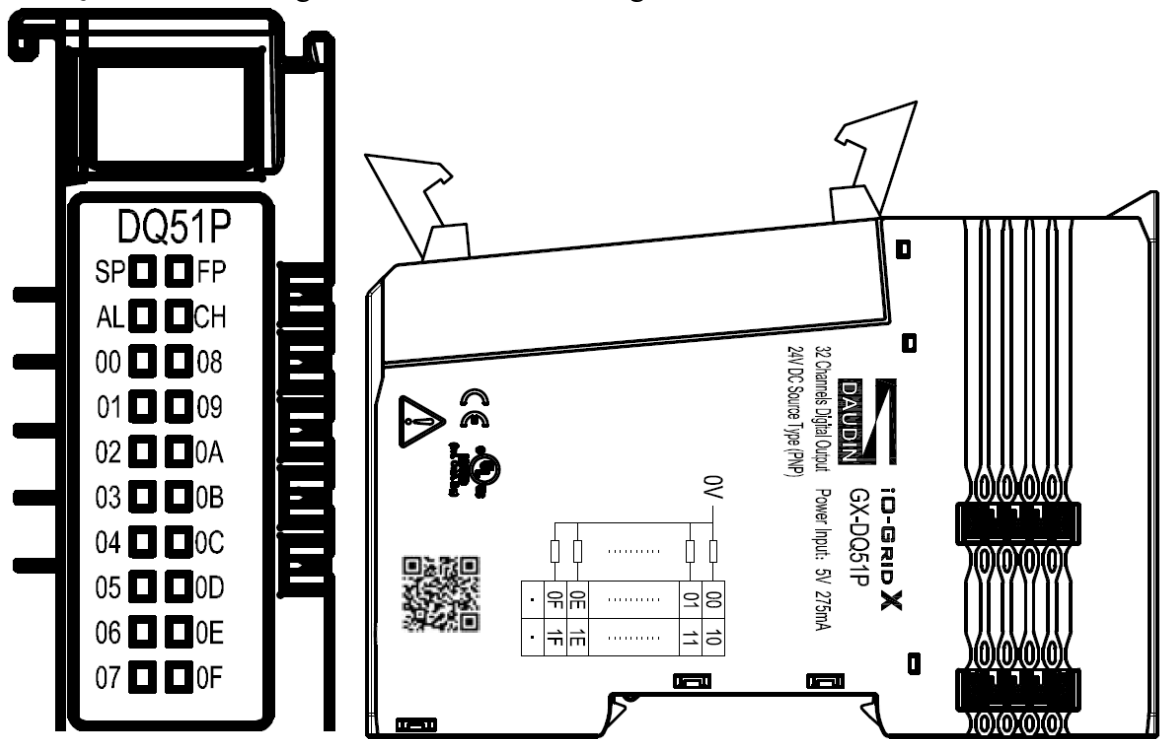
Figure 4.16 GX-DQ51P Diagram
