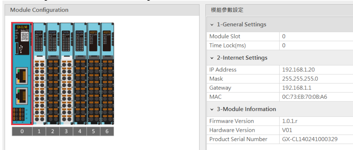
Figure 9.2 Coupler Parameters
