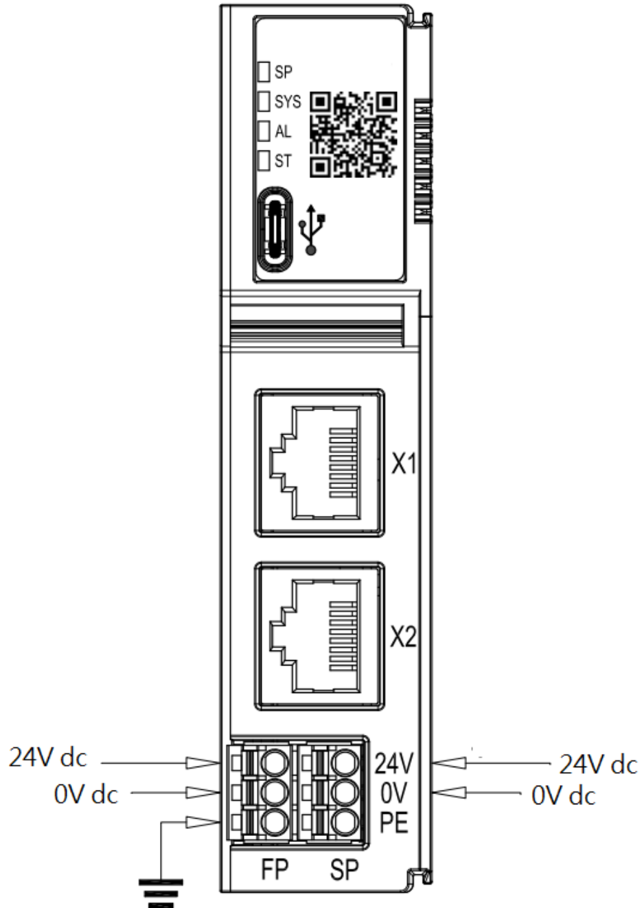
Figure 8.1 Coupler Wiring Diagram
