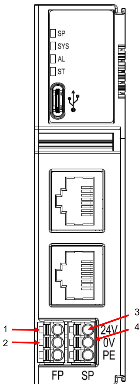
Figure 3.2: Power Supply
