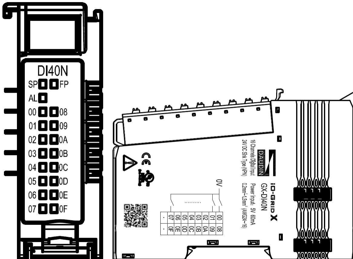
Figure 4.5 GX-DI40N Diagram
