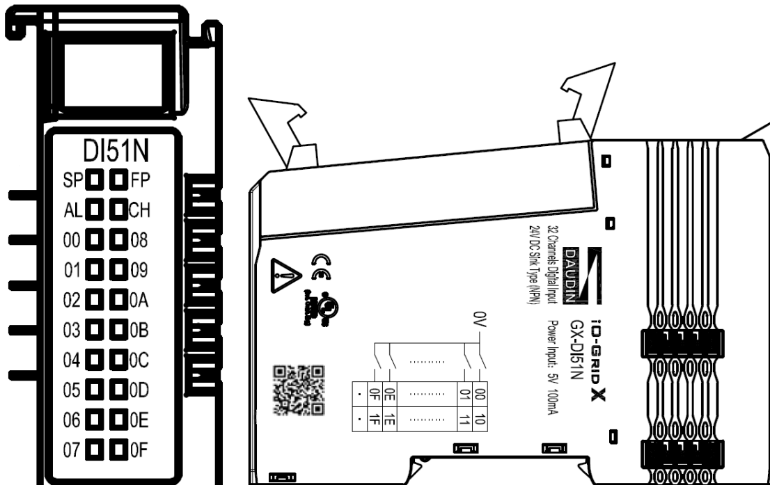
Figure 4.9 GX-DI51N Diagram
