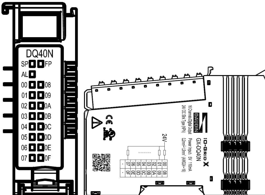
Figure 4.11 GX-DQ40N Diagram
