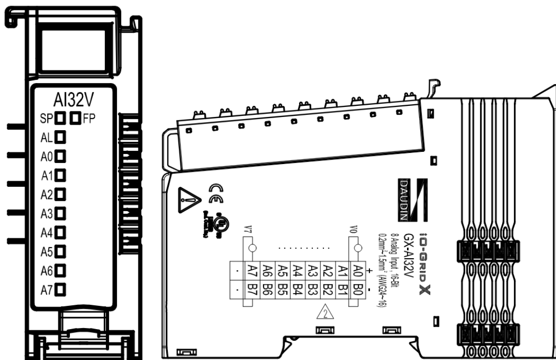
Figure 4.23 GX-AI32V Wiring Diagram
