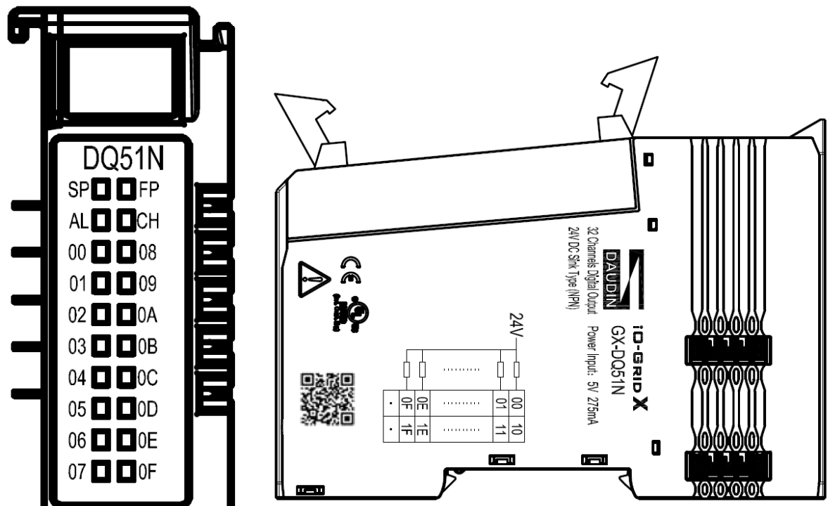
Figure 4.15 GX-DQ51N Diagram
