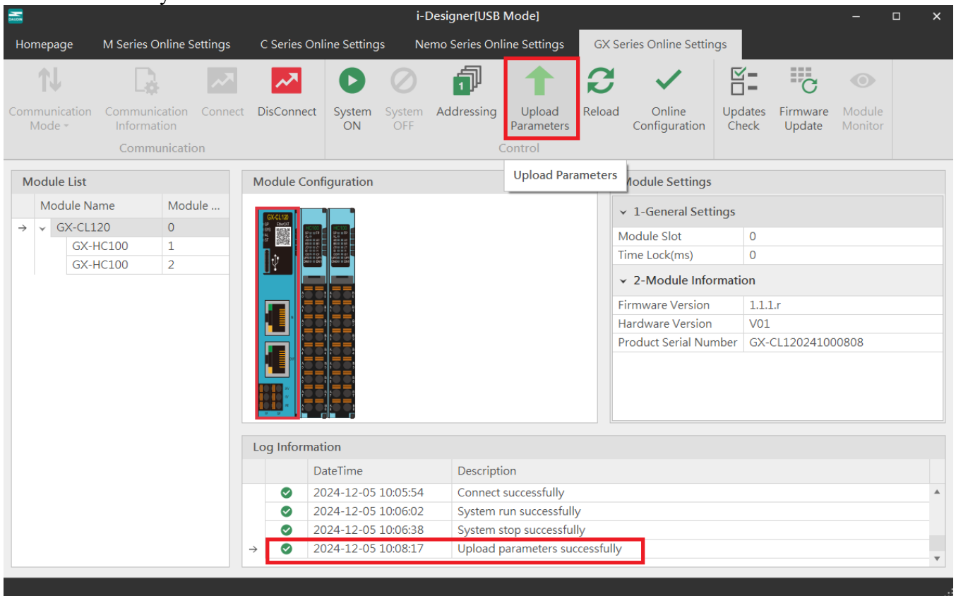
Figure 10.23 Screen After Uploading Parameters
